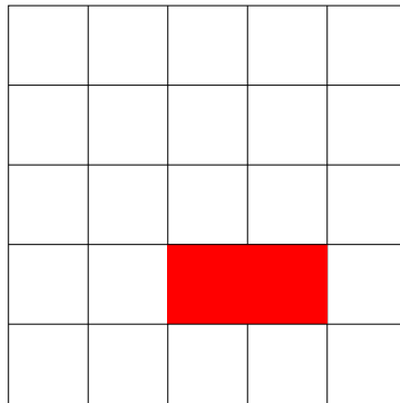
Figure 356: How the Randomized Kruskal's Algorithm Works (2/6)
